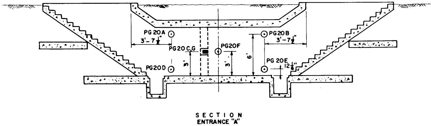
Fig. 2—Gauge locations for entranceway A.
